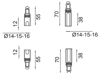
2313 set copricerniere corto con piramide short cover hinges set with pyramid
